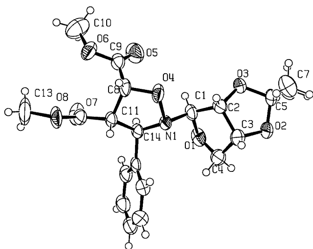
Figure 1. Crystal structure of cycloadduct 12
