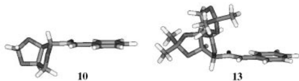
Figure 2. Minimum energy conformers of nitrones 10 and 13
