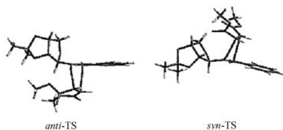
Figure 3. Minimum energy transition-states for the cycloaddition of 10 with 11 ( endo approaches)
